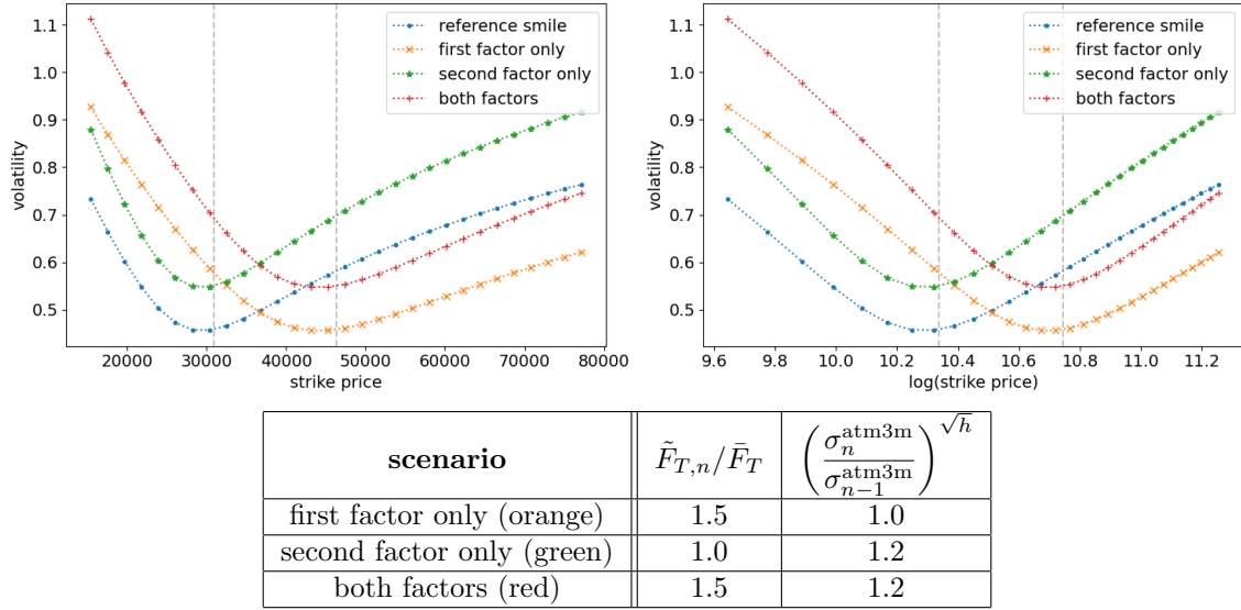
Figure 3: (a) Illustration of volatility simulation model described in equation (3). The reference curve is the 3-month BTC-USD volatility smile as of 2023-07-01, and the simulated smiles are produced by applying each of the corresponding scenarios in the table. In this panel, the smiles are expressed in terms of the strike price. The dashed vertical lines indicate the forward prices before and after the perturbation. (b) Contains the same information, but the smiles are expressed in terms of the log value of the strike price.
