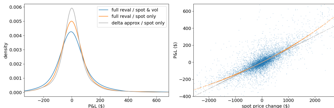
Figure 8: (a) Comparison of the P&L distribution using the full revaluation approach (orange) with that using the first-order delta approximation (grey) assuming only the spot price is simulated. The complete version (blue) of using the full revaluation and simulation of both the spot price and the volatility surface is also shown as a benchmark. (b) Scatterplots of P&L scenarios in terms of simulated spot price changes.
